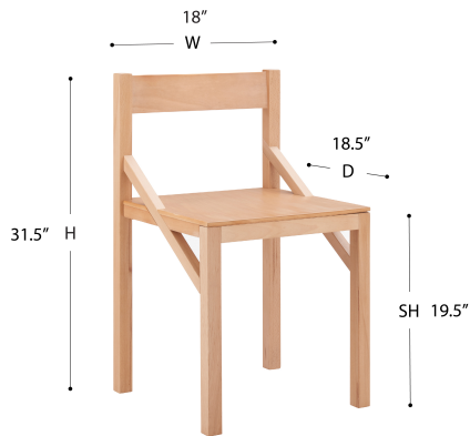
OVERALL DIMENSIONS
